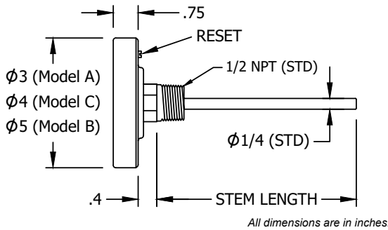
Standard Dimensions
